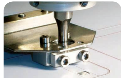
Antenna embedding
